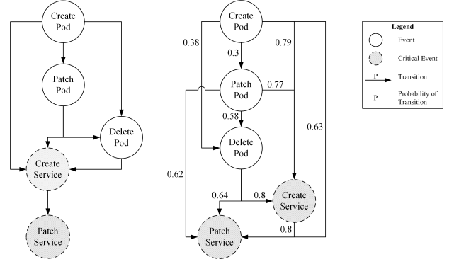
(a) Structure based on immediate transitions (b) Final predictive model based on both immediate and non-immediate transitions
